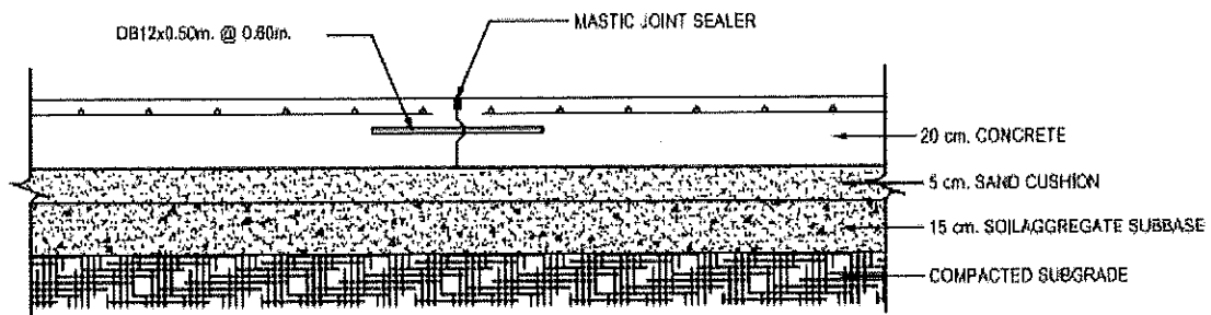
LONGITUDINAL JOINT SCALE 1 : 20
