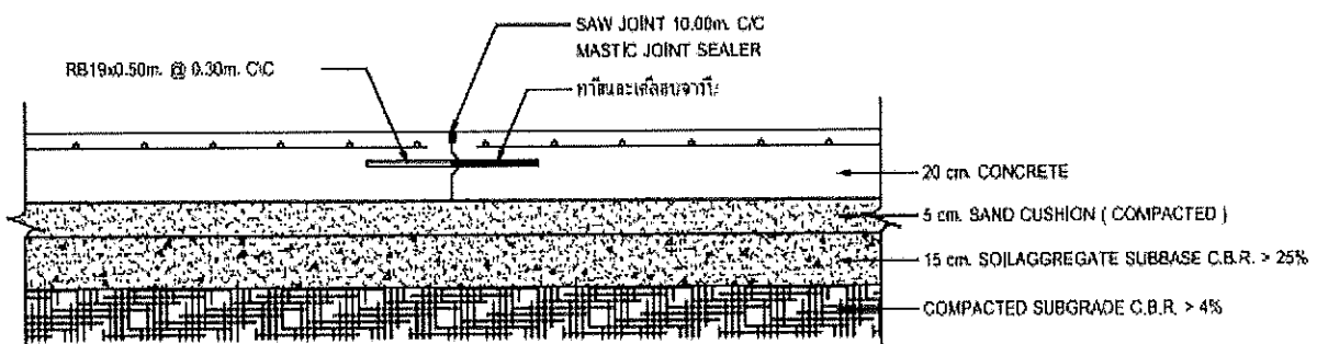
CONTRACTION JOINT
